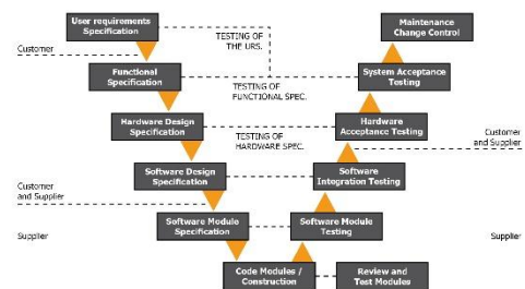
GAMP 5
